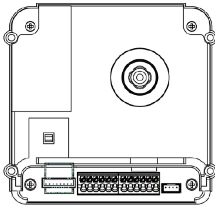
VTO2000A-C Front panel and rear panel
