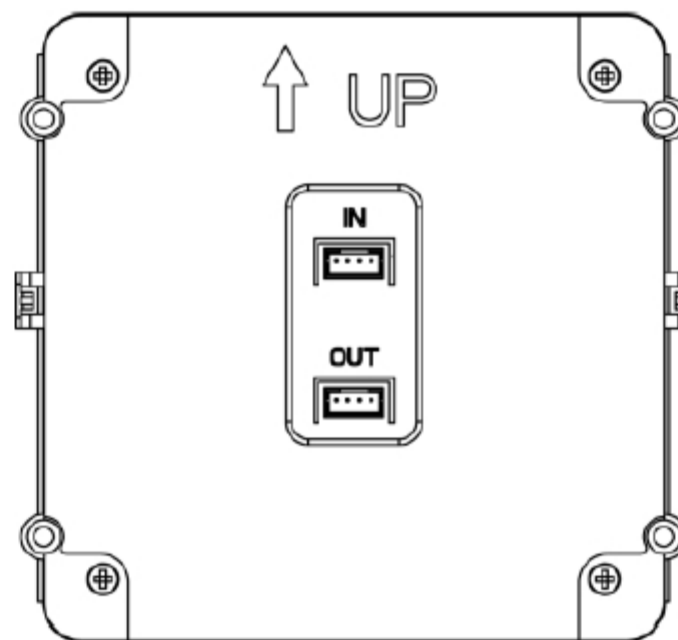
Rear panel
