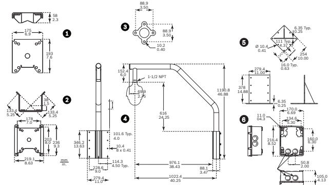
AUTODOME 7000 series Optional Mounts
