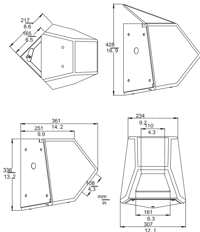
Dimensional Outline
