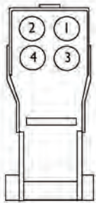
4-pin DC-iris connector (front view)
