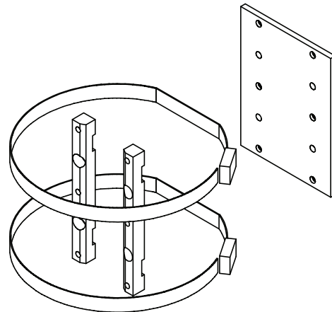
Pole Mount Bracket
