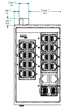
Model SEC418-2SFP-T faceplate detail
