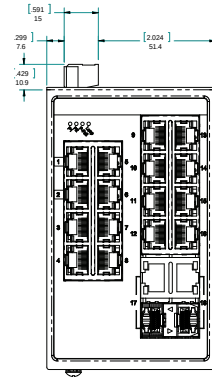
Model SEC418-2SFP-EI-T faceplate detail
