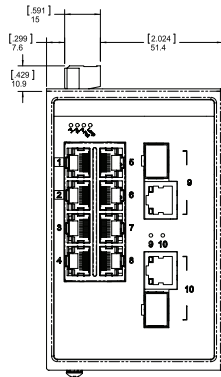
Model SEC410-2SFP-EI-T faceplate detail
