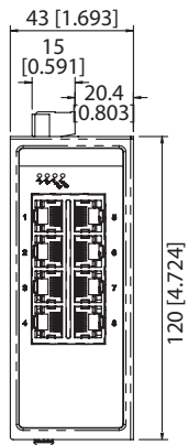
Model SE408-EI-T faceplate detail
