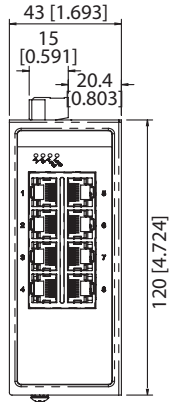
Model SE408 faceplate detail
