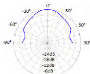
Diagram 2 8" Speaker Polar Plot 2 kHz Octave Band, Grid Spacing = 6dB/Division
