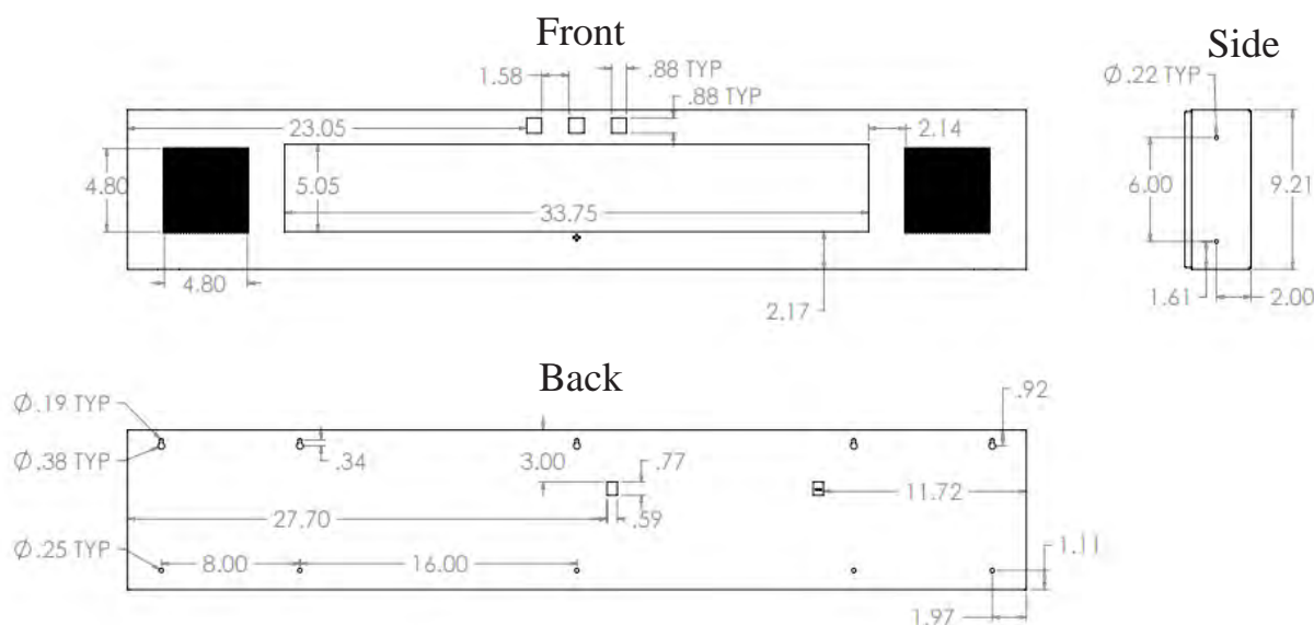
Diagram 1 IPSignl-RWB Dimensions
