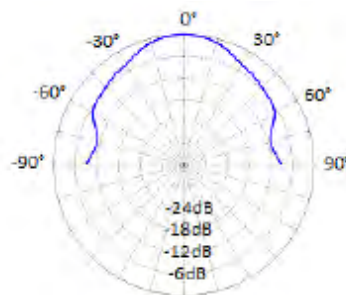
Diagram 2 8" Speaker Polar Plot 2 kHz Octave Band, Grid Spacing = 6dB/Division
