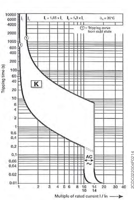
K characteristic
