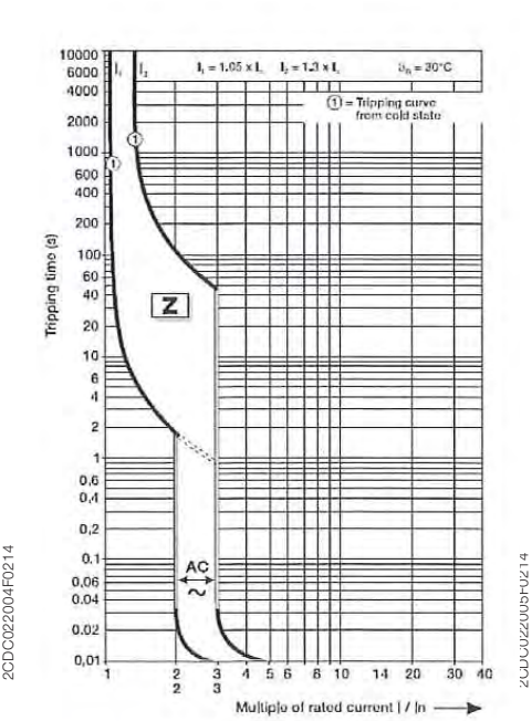
Z characteristic
