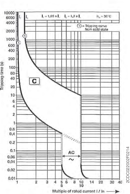
C characteristic
