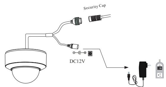
1 Ethernet connector 2 Power connector
