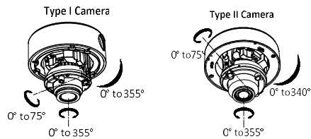
Figure 2-4 3-Axis Adjustment
