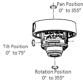
Figure 2-10 3-Axis Adjustment
