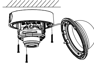
Figure 2-9 Attach the Back Box
