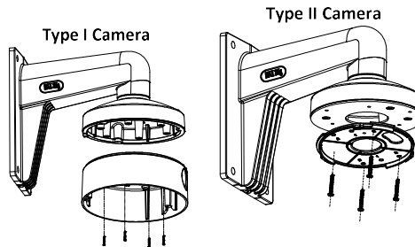
Figure 2-6 Attach the Base Plate to the Mount
