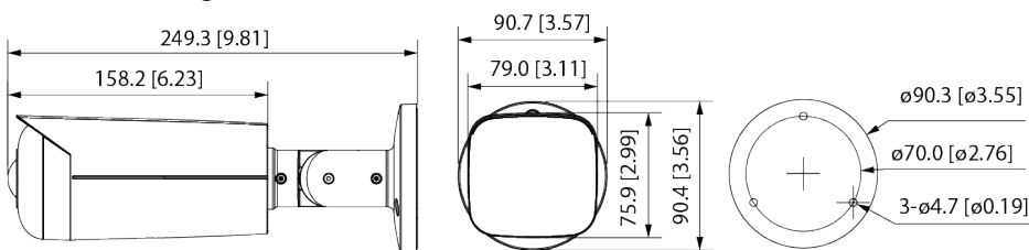
Figure 3-4 Dimensions: Model C (mm [inch])
