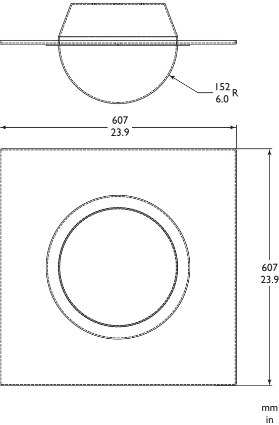
Dimensional Outline - LTC 9312/00
