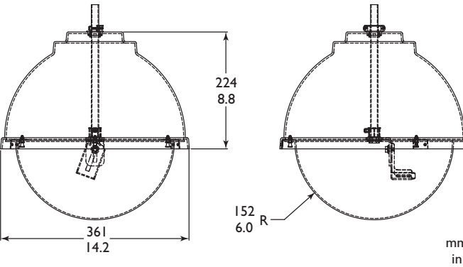
Dimensional Outline -LTC 9412/00
