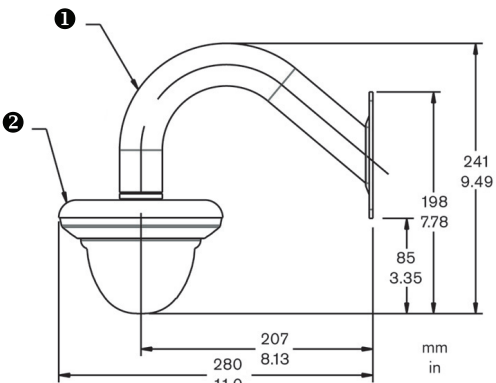
Dimensions LTC 1348/00
