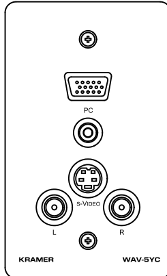
Figure 3: WAV-5YC
