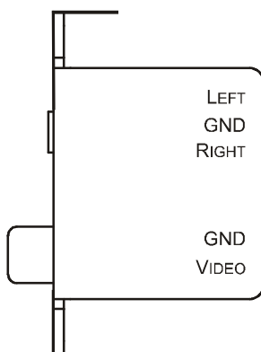
Figure 9: WAV-1R (Side)
