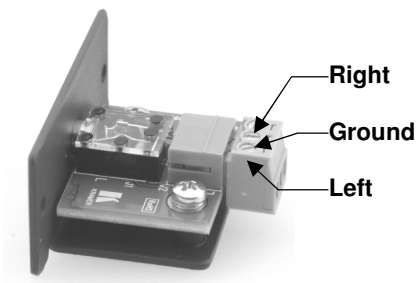
Figure 7: WA-1H (Rear)
