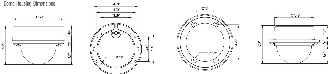
Dome Housing Dimensions
