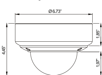
Dome Housing Dimensions
