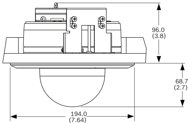
In-ceiling Dimensions
