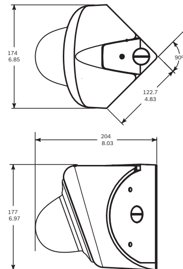
VDA-455CMT-Corner Mount
