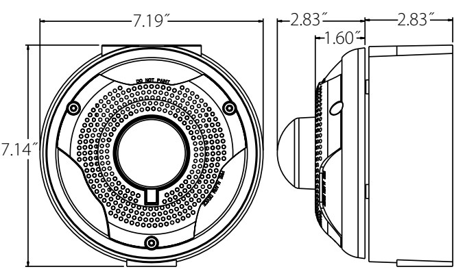
Ceiling-Mount Outdoor Speaker Strobe
