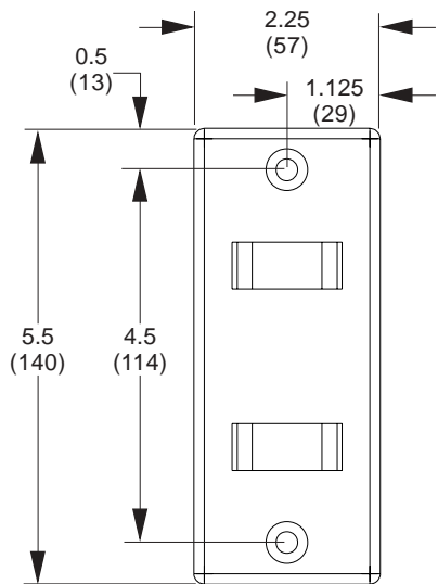
WALL PLATE DETAIL
