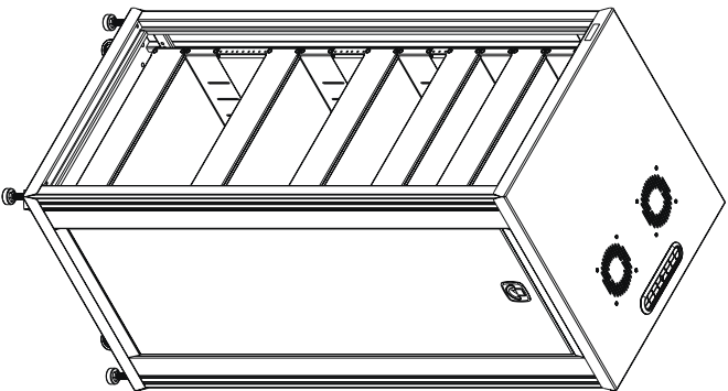
RCS-2724 FACTORY CONFIGURATION (4) 2 SPACE 16" DEEP SHELVES (1) 2 SPACE 18" DEEP SHELF (5) 2 SPACE BLANK PANELS
