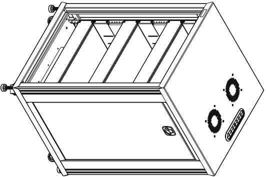
RCS-1824 FACTORY CONFIGURATION (3) 2 SPACE 16" DEEP SHELVES (3) 2 SPACE BLANK PANELS
