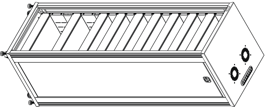
RCS-4224 FACTORY CONFIGURATION (5) 2 SPACE 16" DEEP SHELVES (2) 2 SPACE 18" DEEP SHELVES (2) 3 SPACE 20" DEEP SHELVES (9) 2 SPACE BLANK PANELS
