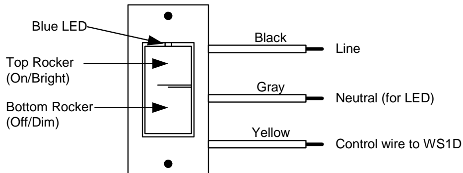
Figure 2: RWS Remote Wall Switch
