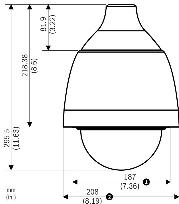
AUTODOME 5000 Dimensions
