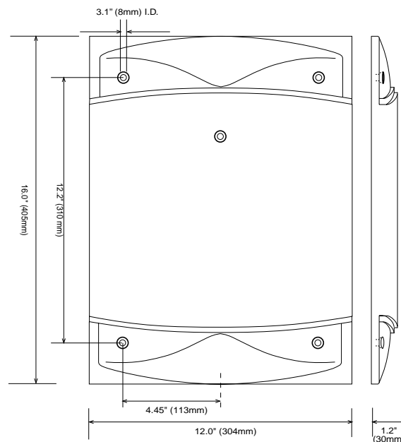
MS-9000 MegaStar Reader
