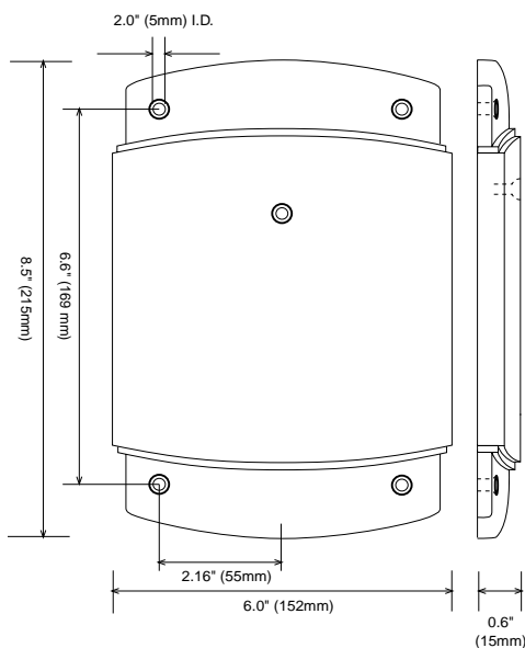
MS-7000 SuperStar Reader
