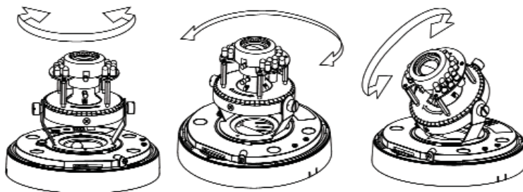
3-Axis Bracket
