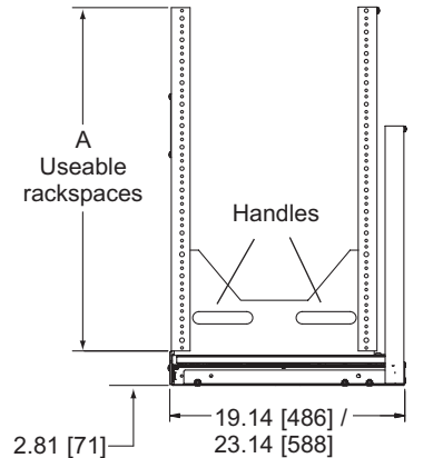
SIDE VIEW CLOSED
