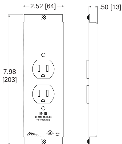
FRONT VIEW SIDE VIEW
