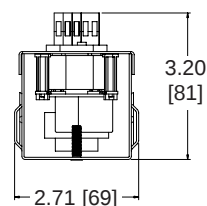
TOP VIEW (module shown installed)
