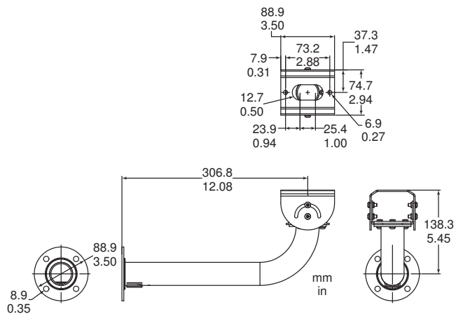
Figure 4: LTC 9215/00 Mount
