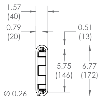
WALL MOUNTING
