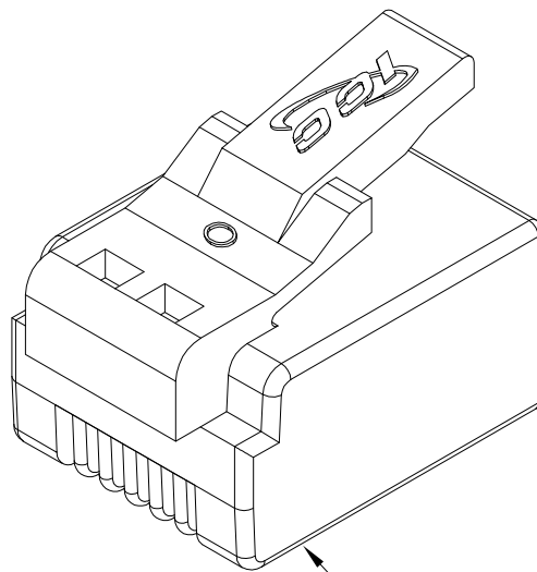
Oval Entry 6P6C Plug
