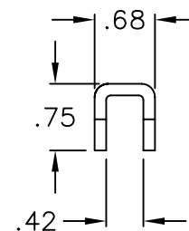
BUTT SPLICE BRACKET
