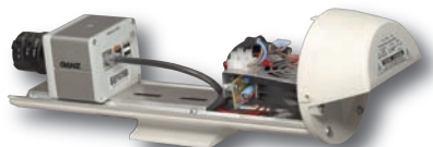
iPak inside view with MPDN Series Camera & 3 Megapixel IR Lens (camera available from 1.3 to 5 megapixels)
