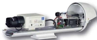
iPak inside view with DDK-1500 Camera & IR Varifocal Lens
