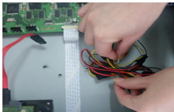
Unfasten the HDD power cable.
