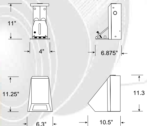
Anchor plate with camera mounting
