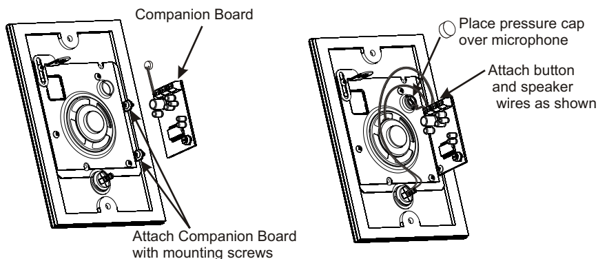
Completed Sub-assembly
