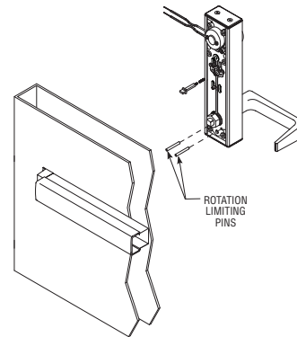
Cylinder and Solenoid Installation
