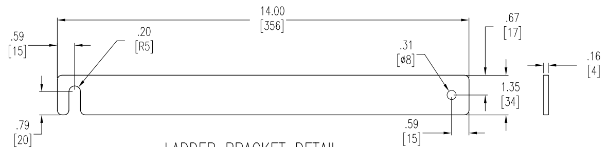
LADDER BRACKET DETAIL
