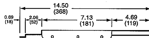
TOP VIEW RH BRACKET
