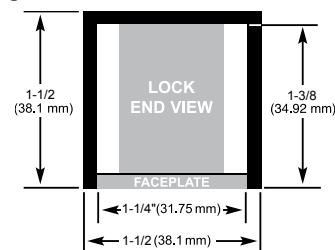
Figure 4: End View
