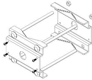
AN-ACC-AP-O- POLE Access pole mount sold separately
