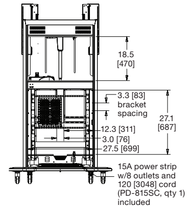
rear view (rear doors removed and bottom hidden for clarity)
