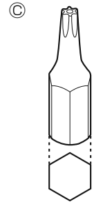
Hex wrench, screw size 6.35 mm {1/4 inches} T10
