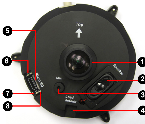
Figure 1-2a: GV-FE Series
