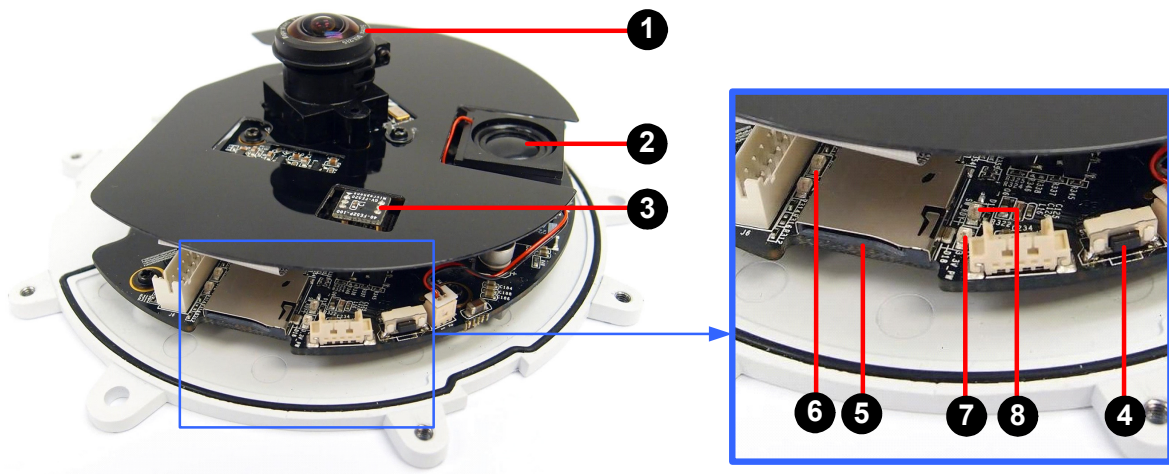
Figure 1-2b: GV-FER521
